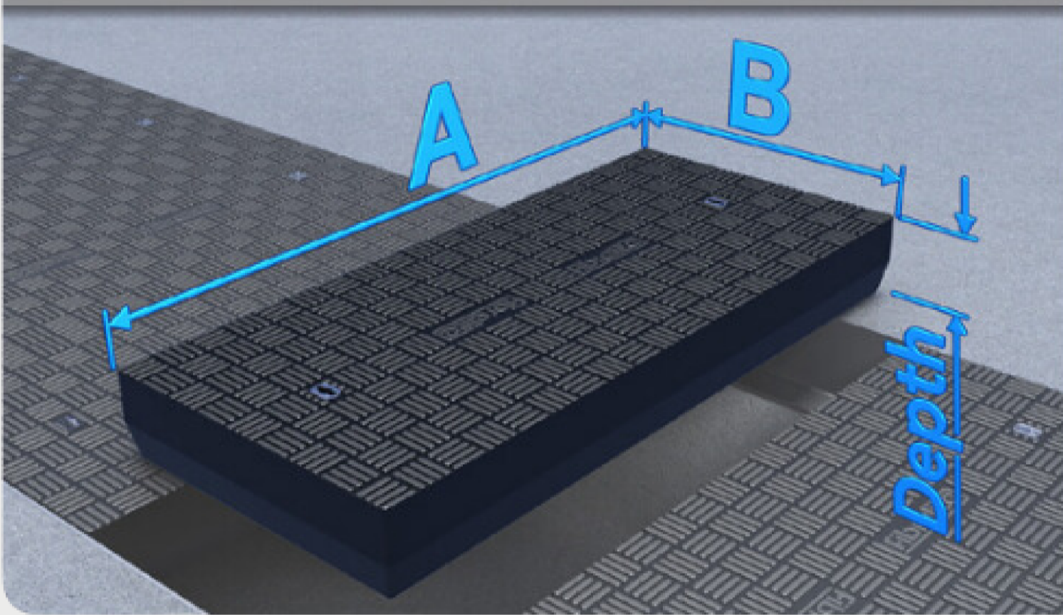
Trench widths over 1m (40") up to 1.6m (64")
