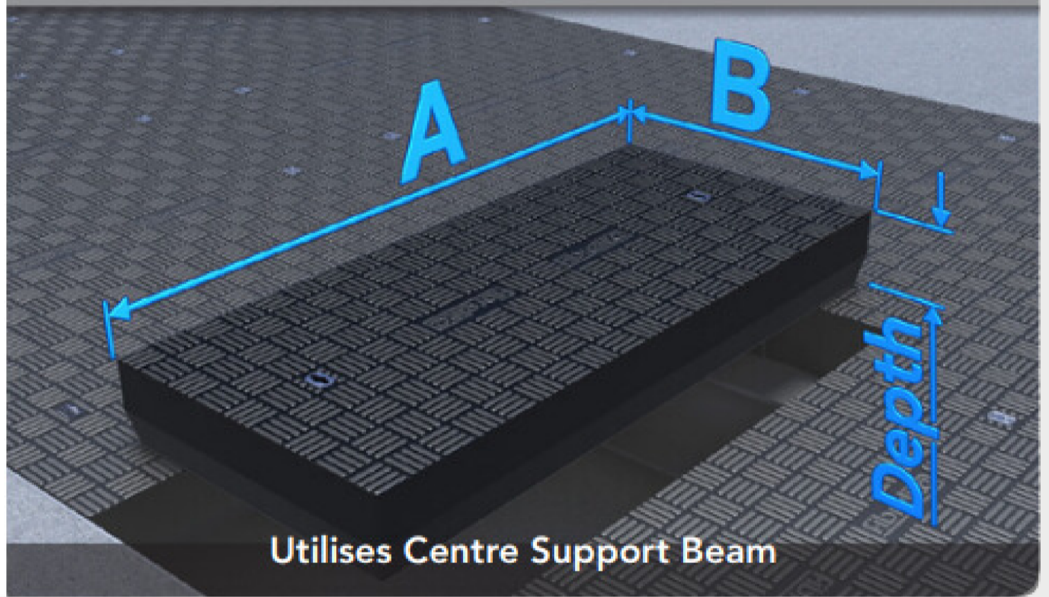
Trench widths over 1.6m (64")
